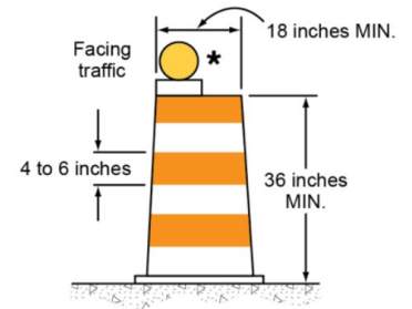
Drum for use with the Type 3 Barricade
