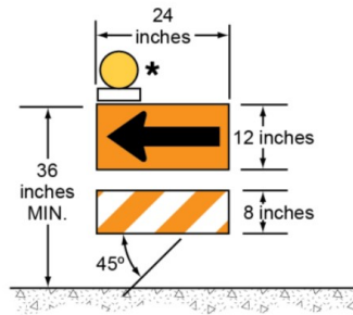
Direction Indicator Barricade
